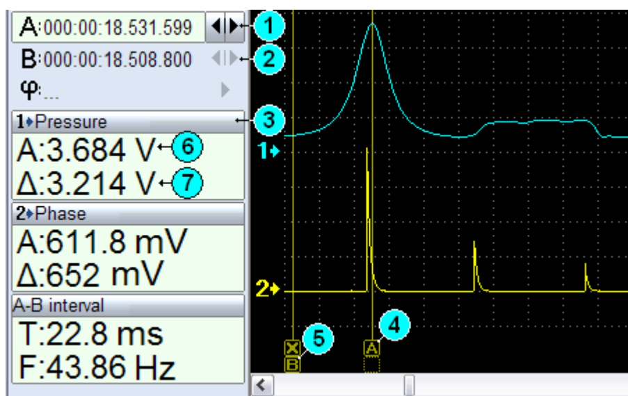
fig. 19. Measurement panel and A and B markers.
