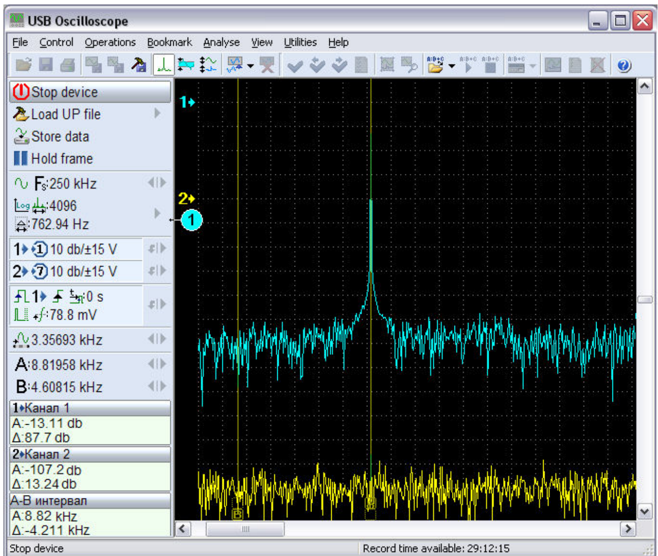
Fig. 8. Program window in specter mode
