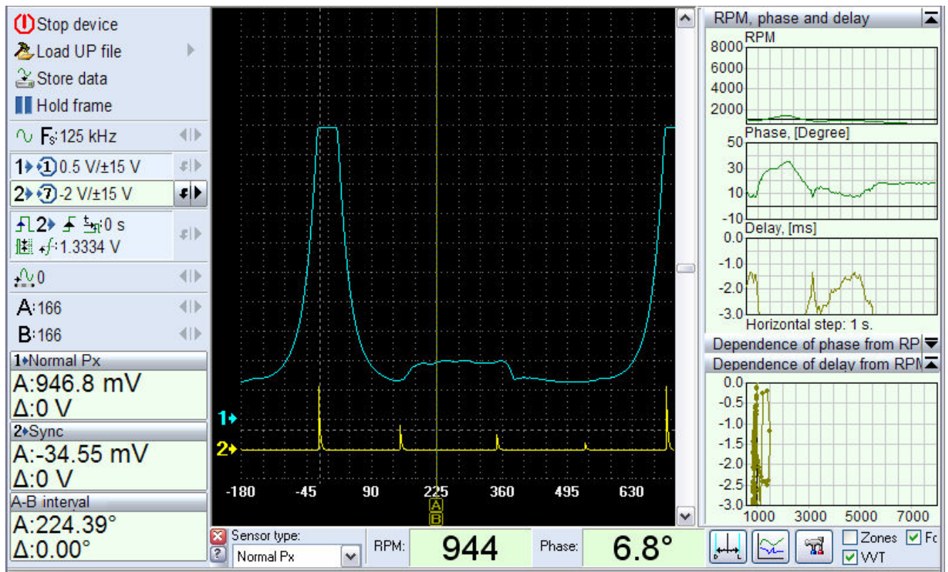
fig. 27. Program window when plug-in is loaded.
