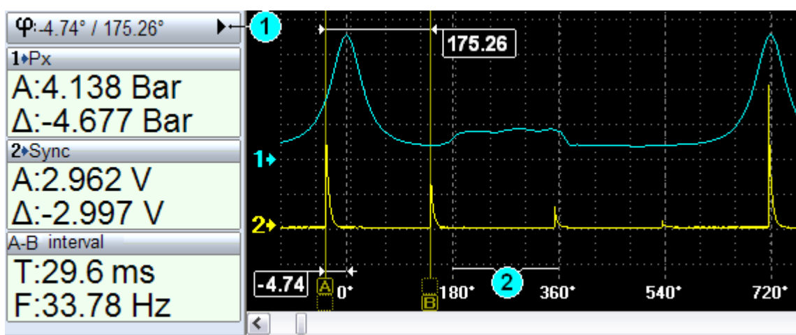
fig. 20. Phase measurement.
