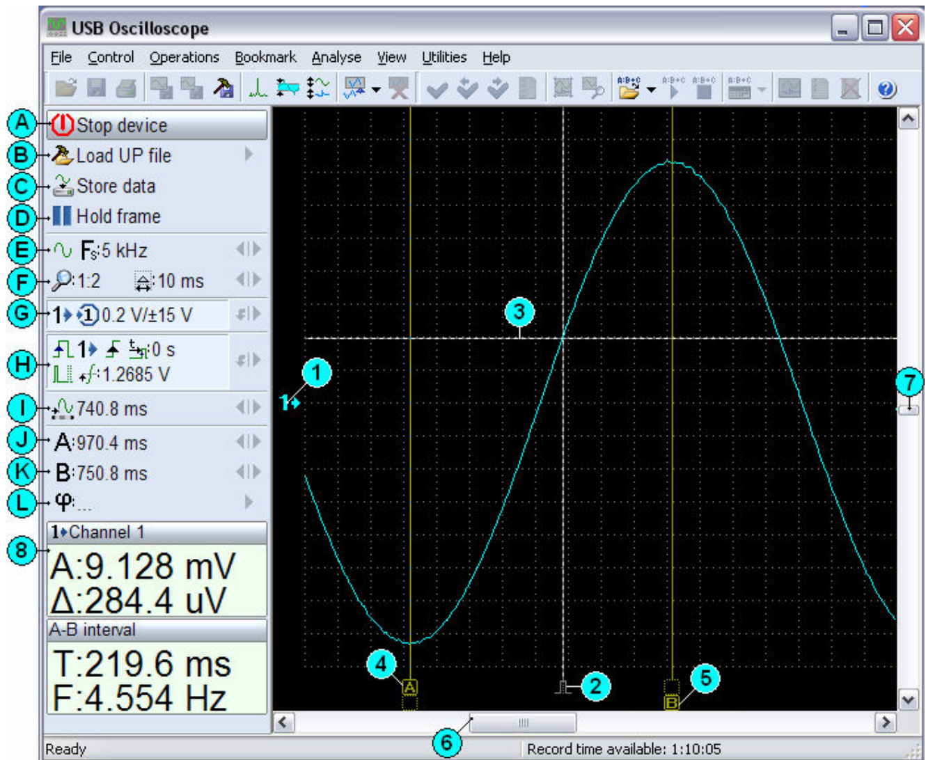
fig. 4. Program window in analogue oscilloscope mode
