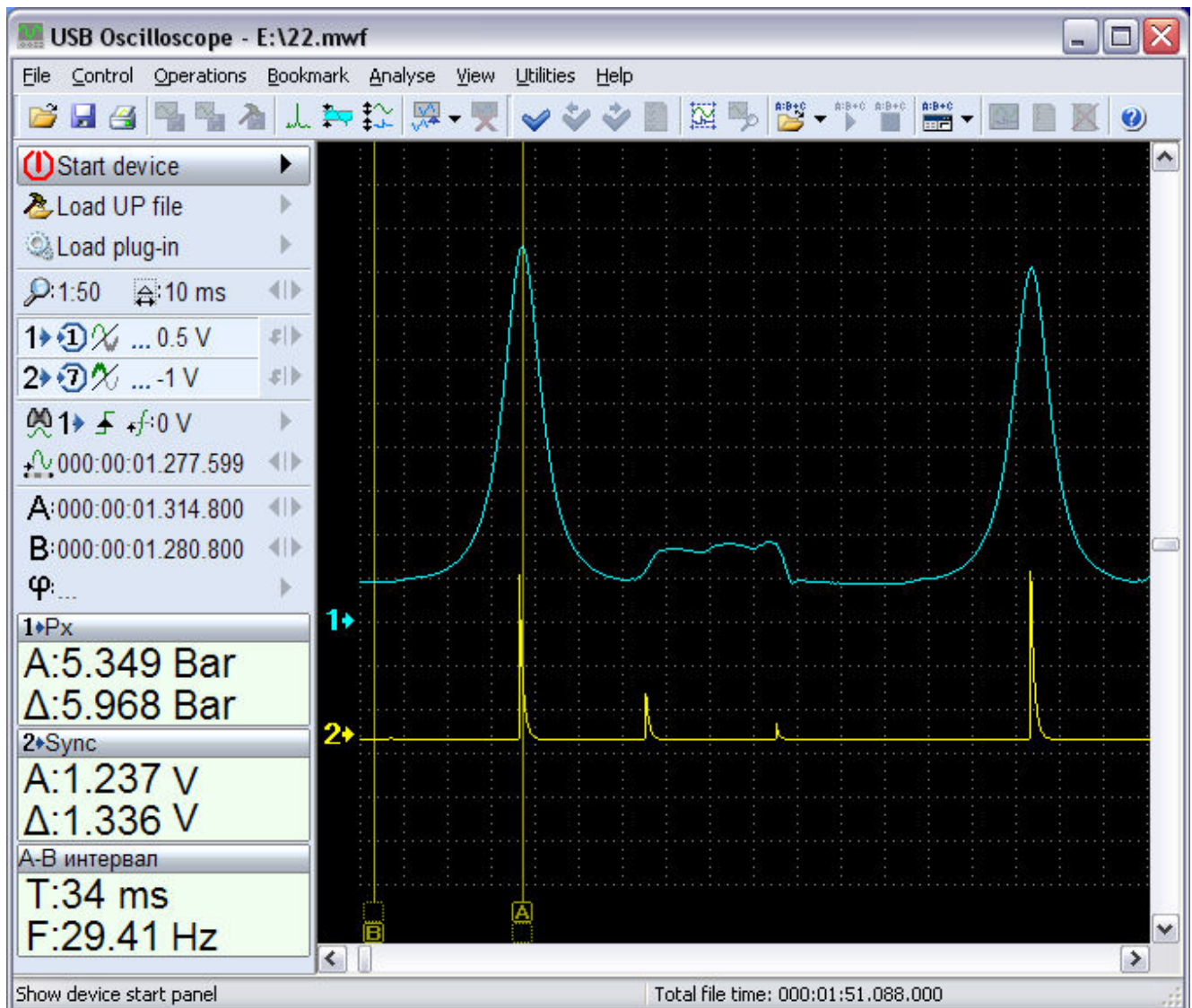
fig. 13. Program window in oscillogram view mode.
