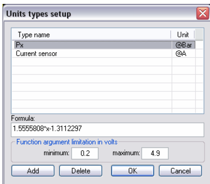
fig. 22. “Units types setup” dialog.
