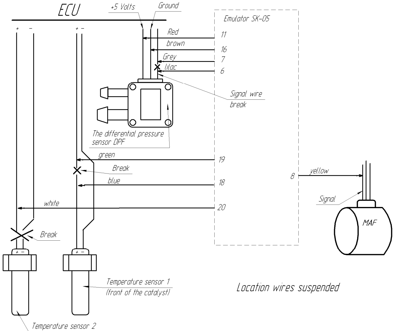
Figure 3.1. Scheme of connection of emulator SK-05 with 2 temperature sensors.
